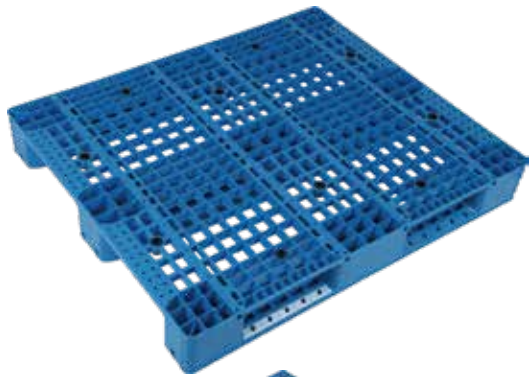
QUA-CZP01 1000*800*150mm Stack load: 4 T Dynamic load: 1 T
