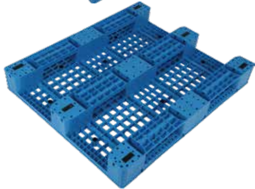
QUA-CZP03 1200*800*155mm Stack load: 6 T Dynamic load: 1.5 T
