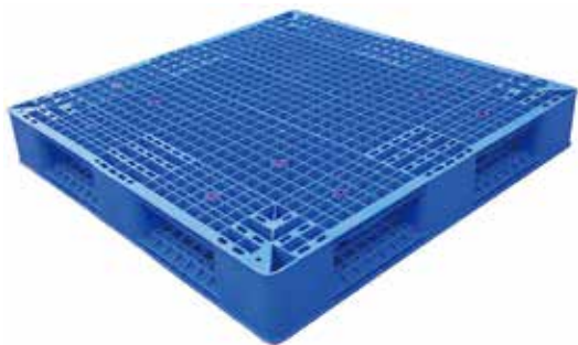
QUA-TZP01 1000*1000*150mm Stack load: 4 T Dynamic load: 1 T
